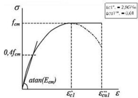
Fig.No.05 Constitutive relation for the concrete
