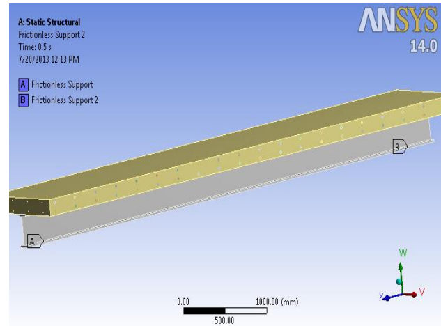
Fig.No.09 Boundary condition and support linkages
