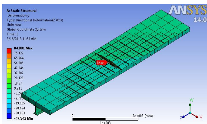
Fig No.12: Cracking on slab due to concentrated force.
