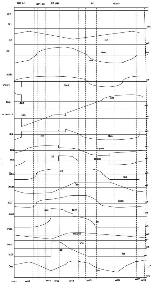
Fig 2.0 Operating modes of proposed current fed isolated LLC-T Resonant converter
