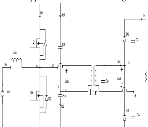
Fig 1.0 Schematic of proposed Isolated Soft switching Current fed LCC-T Resonant DC-DC converter
