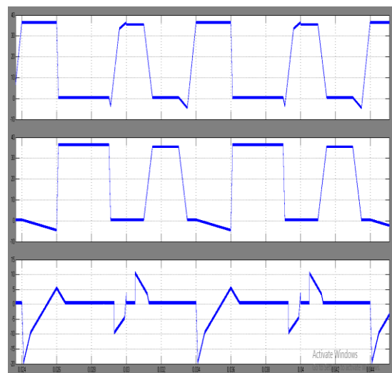
Fig.3 simulation results for converter subjected to wide load variations and input voltage variations
