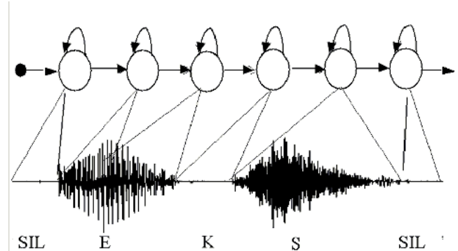
Figure 7: Hidden Markov model
