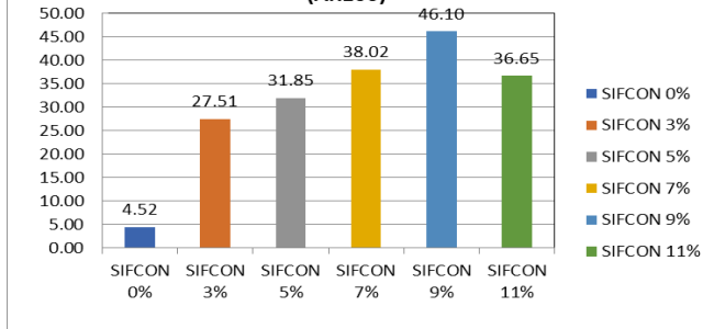
Figure 6. Flexural Strength in MPa at 28 Days for different SIFCON % (AR100)
