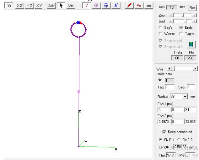
Figure 2 – Simulation of antenna.
