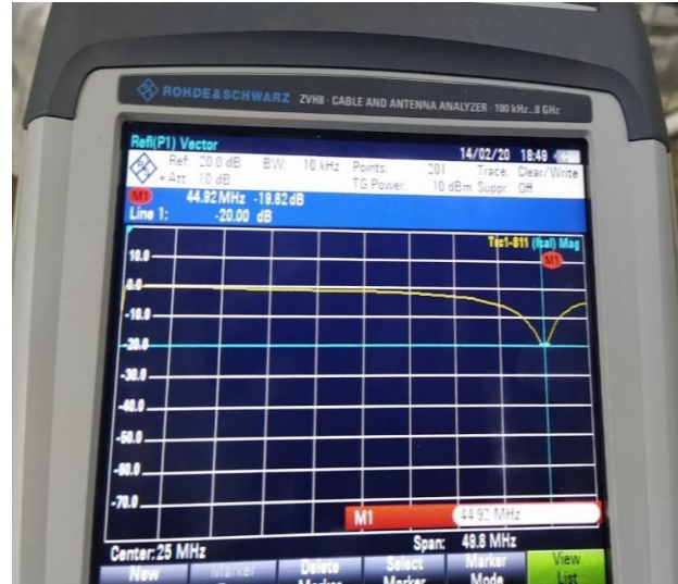
Figure 6- Antenna response (Tuned at 44.92 MHz)
