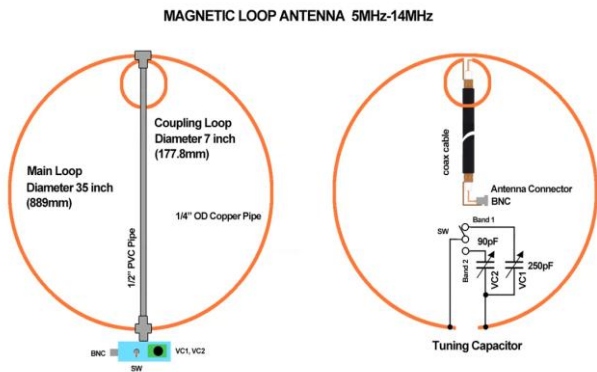
Figure 1 – Construction of Magnetic Loop Antenna
