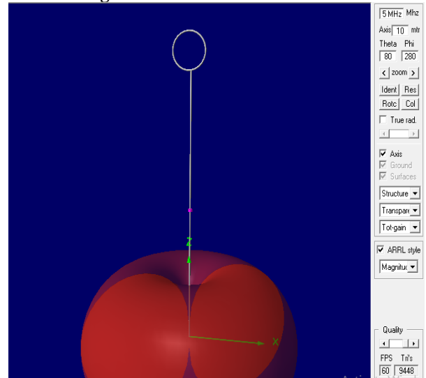
Figure 3-Simulation of antenna with 3D field pattern.
