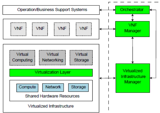
Fig. 2: NFV tectonic structure
