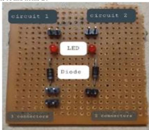
Fig. 2. PCB Board for charging circuit
