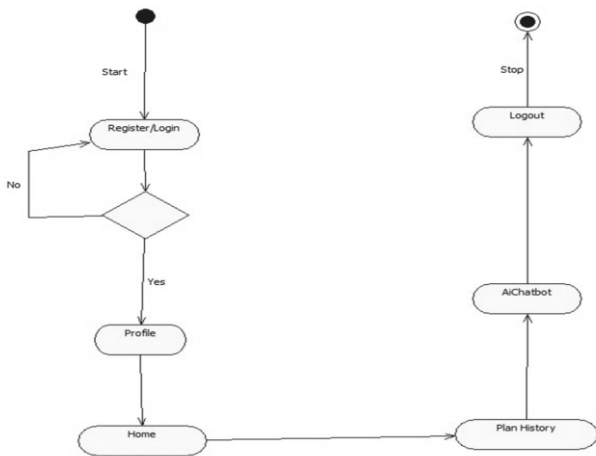
Fig.2. Activity Diagram
