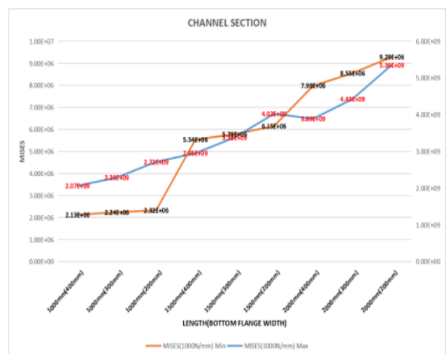
Fig. 14. MISES in C Section under 1000N/m
