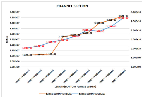
Fig. 16. MISES in C Section under 5000N/m
