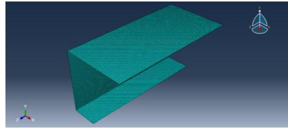
Fig.8. FEM meshed model
