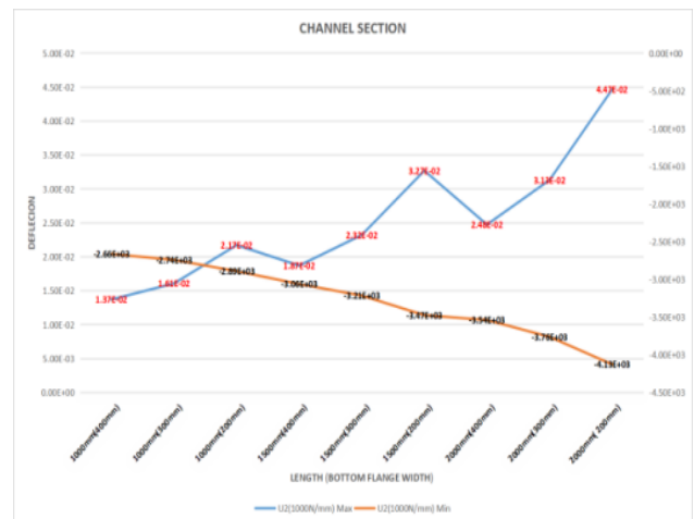
Fig. 13. Deflection in C Section under 1000N/m
