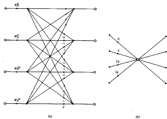
Fig 3: Radix 4 butterfly
