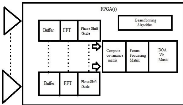
Fig 2: CSSM Algorithm
