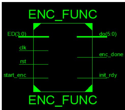
Encoder Block
