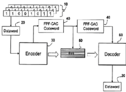
Fig1: Block diagram of our proposed system
