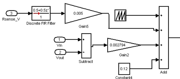
Fig.3 Digital PWM control for Buck Mode Operation
