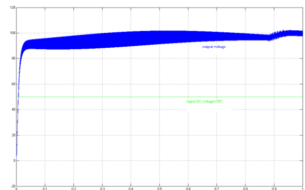
Fig.7(c) Purposed PBB converter output voltage Waveforms (Input V_{dc}=50V )
