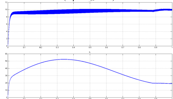
Fig.7(b): Waveforms for I_{out} and I_L (Input V_{dc}=50V )
