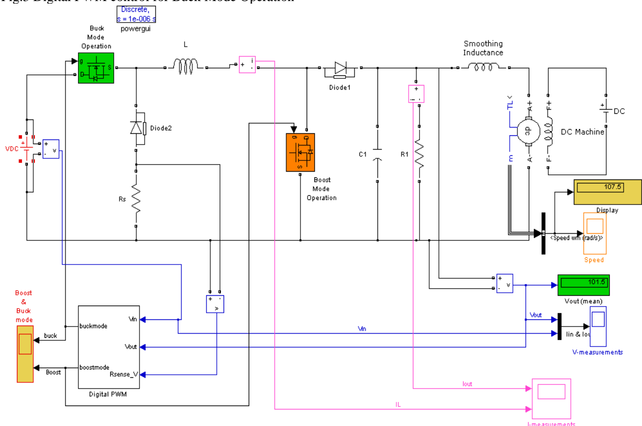
Fig.5 Digital PWM control PBB converter
