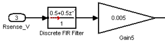
Fig.1 R_{sense} loop for Digital PWM Signal
