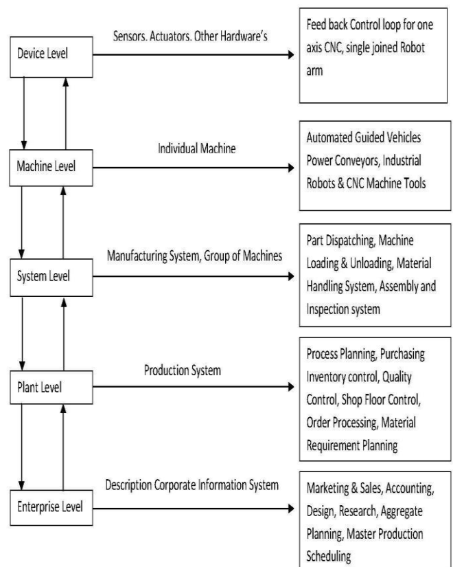
Fig.3 Five Levels of Automation in Manufacturing
