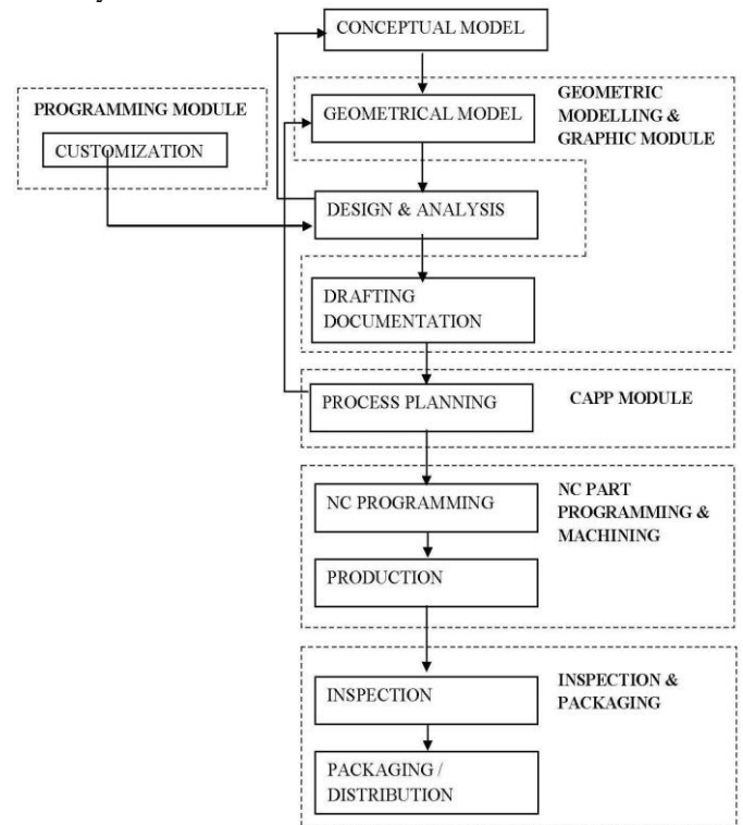
Fig.7 A CAD/CAM Modules in Industry
