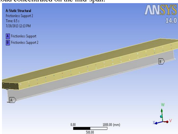
Fig.No.09 Boundary condition and support linkages
