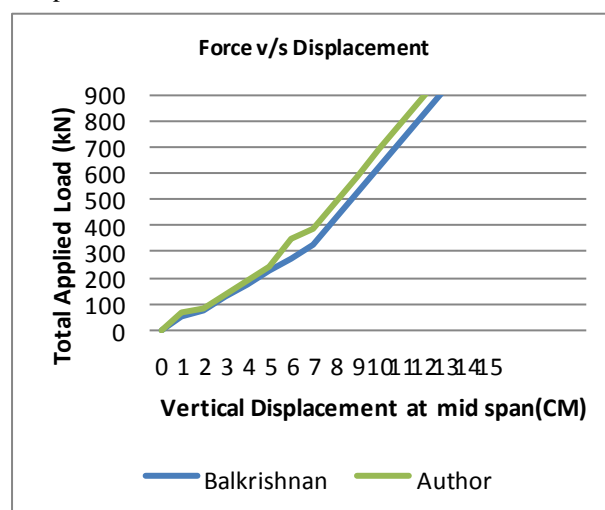
Graph No. 01(a): Graphical Force v/s Vertical Displacement
