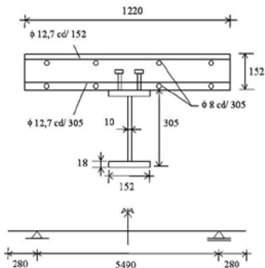
Fig No. 02 Dimensions of Composite beam model
