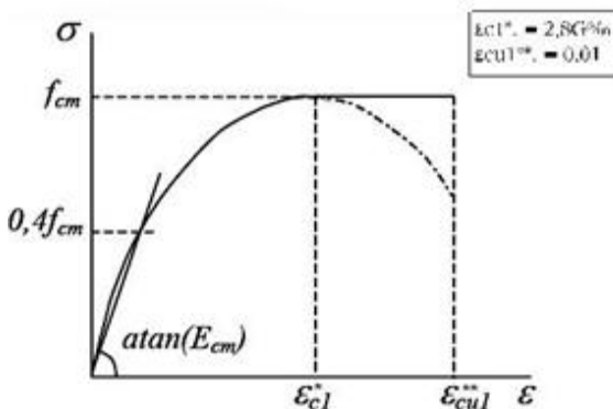
Fig.No.05 Constitutive relation for the concrete
