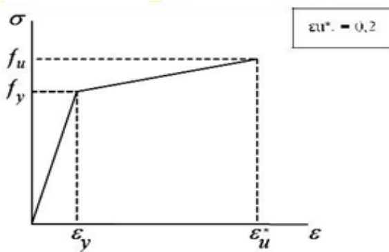
Fig No. 07 Constitutive relation for the shear connectors (10)
