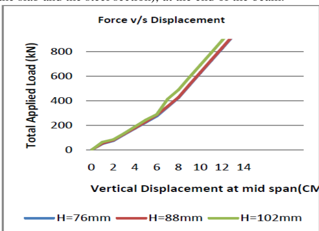
Graph No. 02(a) Graphics Force v/s displacement to connectors with 19mm \Phi (AUTHOR)
