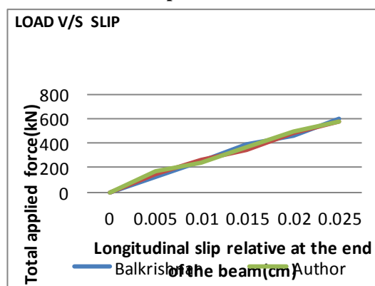
Graph No. 01(b): Force v/s Slide of A3 Beam
