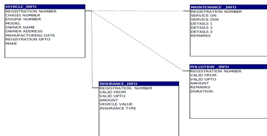
Fig6.1: E-R DIAGRAM FOR HSVP DATABASE
