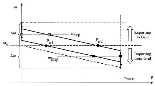
Figure 2 Power Vs Frequency Droop
