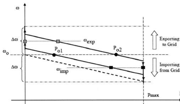
Figure 2 Power Vs Frequency Droop
