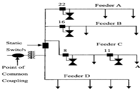
Figure 1 Basic microgrid Architecture Diagram
