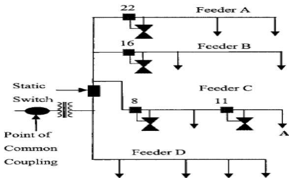
Figure 1 Basic microgrid Architecture Diagram
