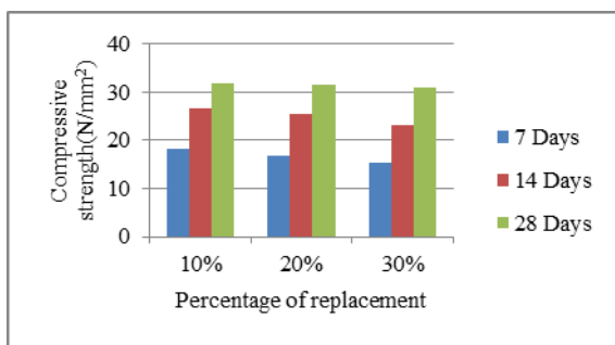
Fig. 1. Compressive strength of stone dust replacement
