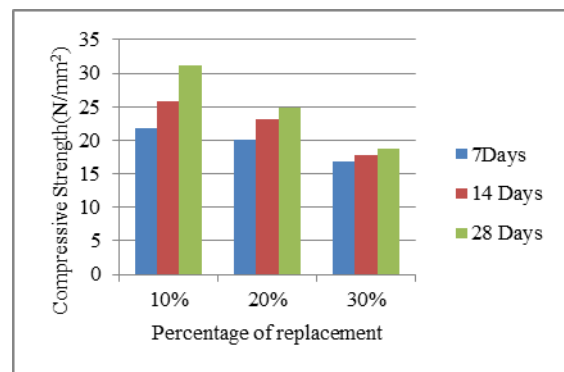
Fig. 4. Compressive strength of Fly Ash replacement.
