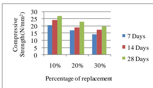
Fig. 3 Compressive strength of coconut shell replacement
