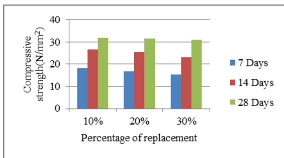
Fig. 1. Compressive strength of stone dust replacement
