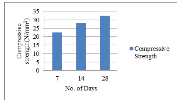
Fig.1 Compressive strength of Referral Concrete
