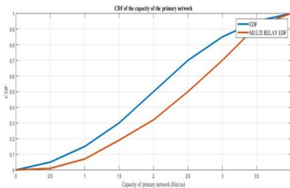
Fig.3: CDF of Primary Network Capacity
