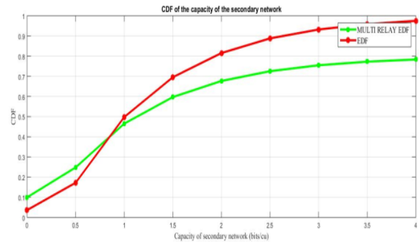
Fig.4: CDF of Secondary Network Capacity
