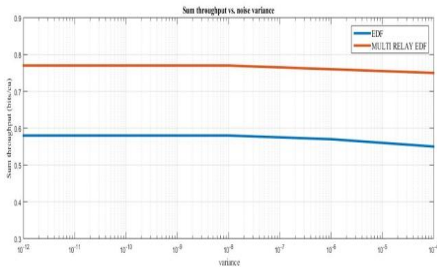
Fig.7: Sum Throughput over Variance
