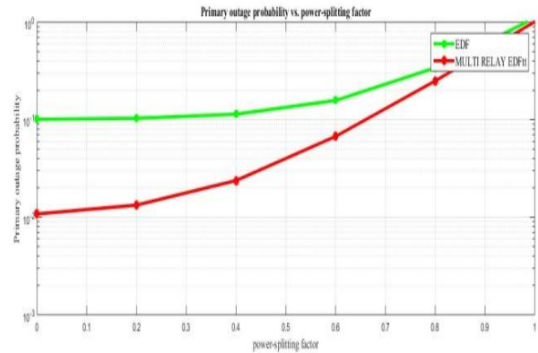
Fig.5: Primary Outage Probability over Power splitting factor
