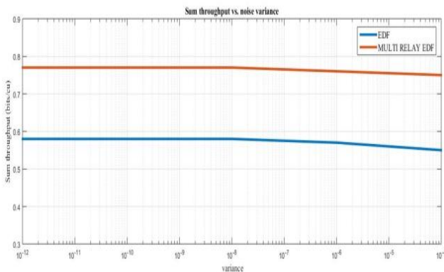
Fig.7: Sum Throughput over Variance
