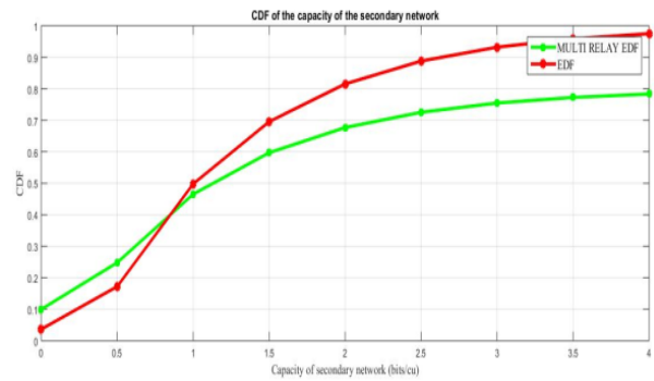
Fig.4: CDF of Secondary Network Capacity
