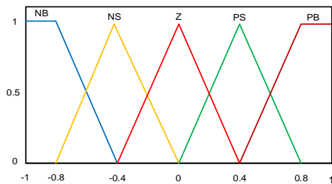
Figure 6 Membership function for input and output.
