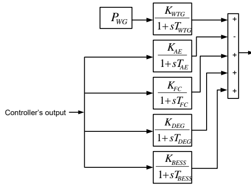
Figure 19 (c) Transfer function model of DG units.
