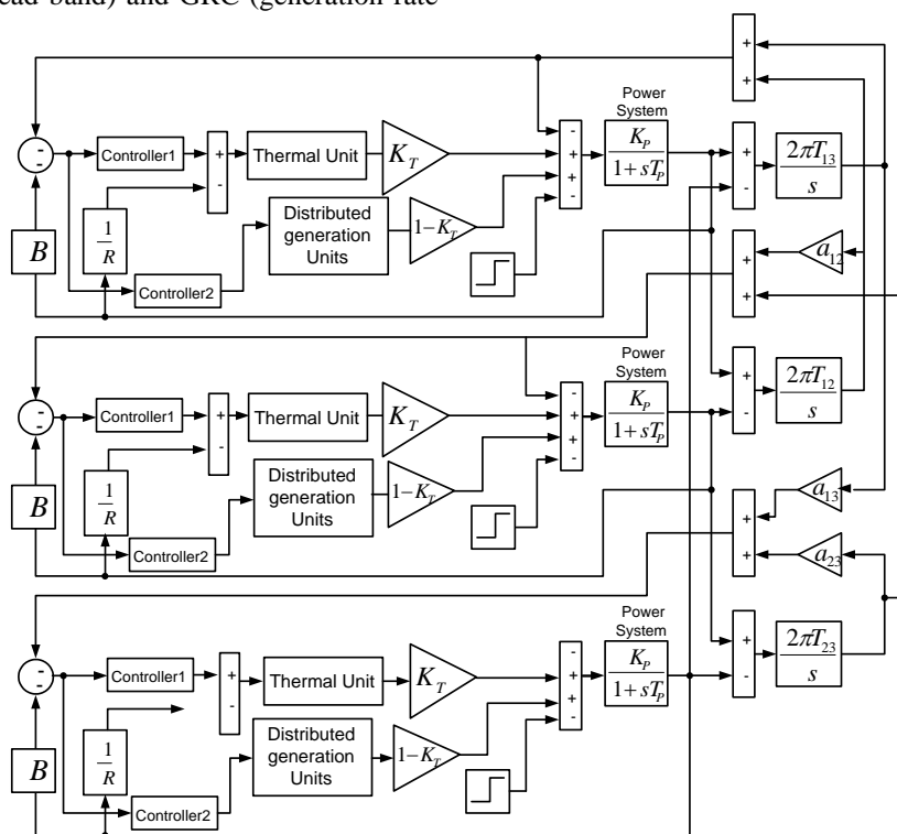
Figure 19 (a) Transfer function model of three area system.
