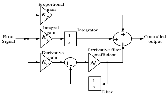
Figure 3 Structure of PID controller with derivative filter (PIDF).
