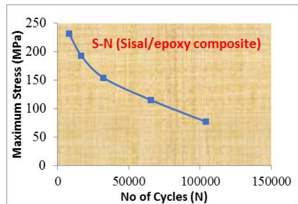
Fig.3. S-N Curve Of Sisal Fiber Composite
