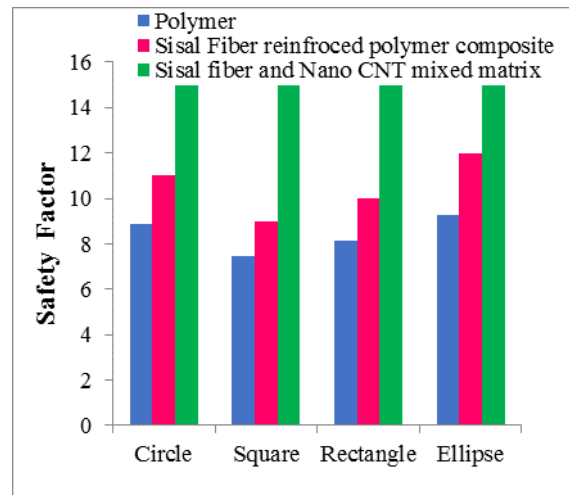
Fig.10. Safety Factor Of Composite With Different Irregularities
