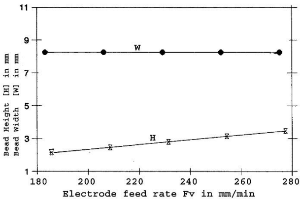
Fig.13 Effect of electrode feed rate on bead height and bead width keeping other parameters constant
