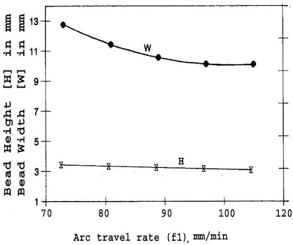
Fig.12 Effect of arc travel rate on bead height and bead width keeping other parameters constant
