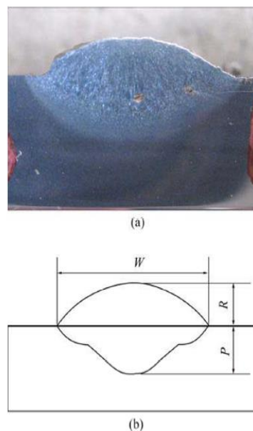
Fig. 6 (a) Weld bead cross section (b) Weld bead geometry
