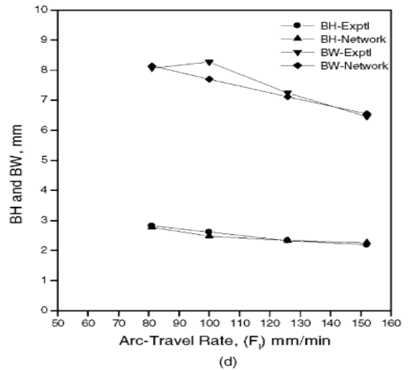
Fig. 3. Bead height (BH) and Bead width (BW)
