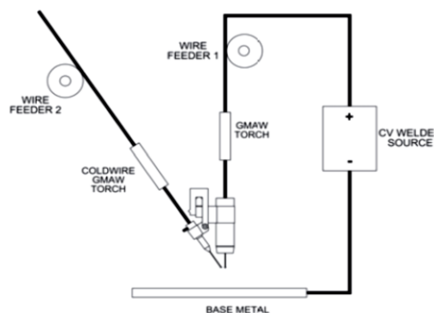
Fig. 7. General Scheme for CW GMAW
