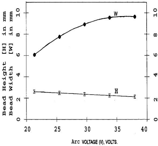
Fig.11 Effect of arc voltage on bead height and bead width keeping other parameters constant
