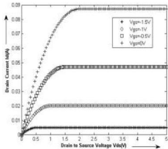
Fig.5. I_{ds} Vs V_{ds} simulation response of 3C-SiC MESFET.
