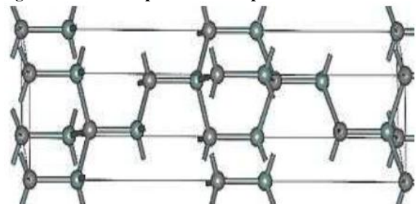
Fig.2. 3D dimensional periodic cell representation of 4H-SiC.
