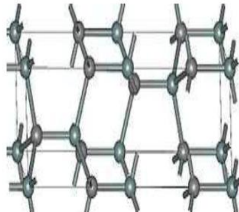
Fig.2. 3D dimensional periodic cell representation of 4H-SiC.
