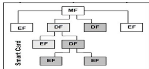
Figure 4. Smart Card File System /DF: Dedicated File / MF: Master File / EF: Elementary File
