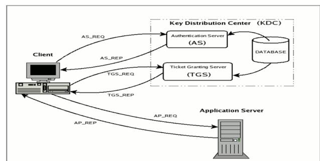
Figure 2. Kerberos authenticated Service Provision Architecture.
