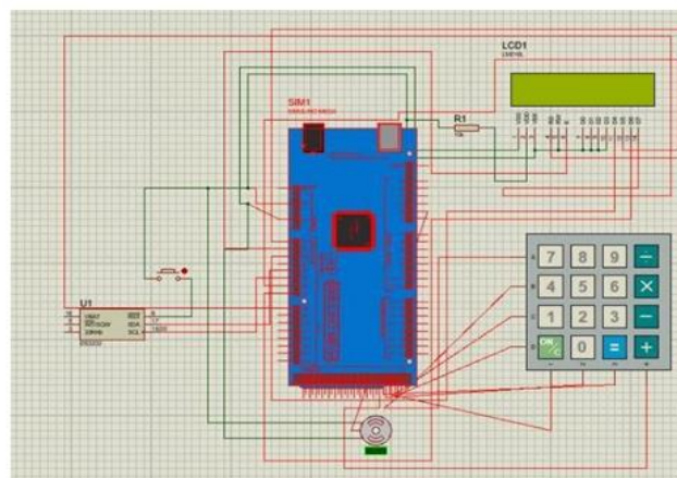
Fig. 2. Circuit diagram of the proposed system
