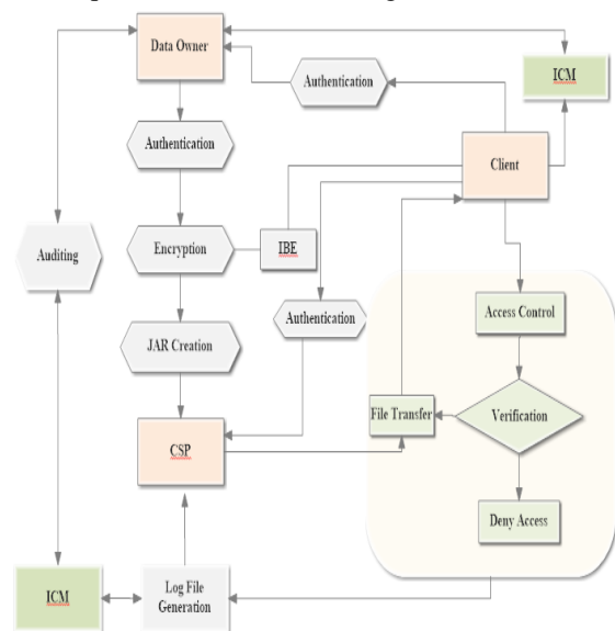
Figure 4: Data Flow of the Proposed Work
