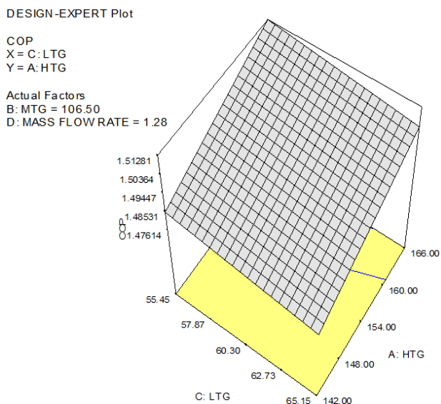
Figure 2. 3D surface plot of COP vs LTG vs HTG.
