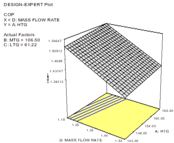
Figure 4. 3D surface plot of COP vs MFR vs HTG
