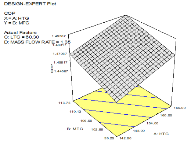
Figure 3. 3D surface plot of COP vs MTG vs HTG
