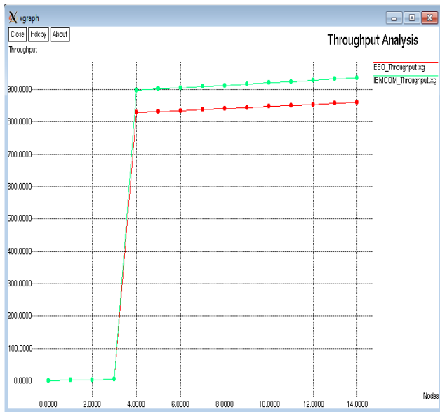
Fig.6 Throughput Analysis
