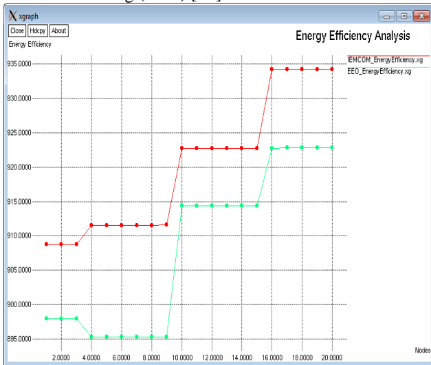
Fig.7 Energy-Efficiency Analysis
