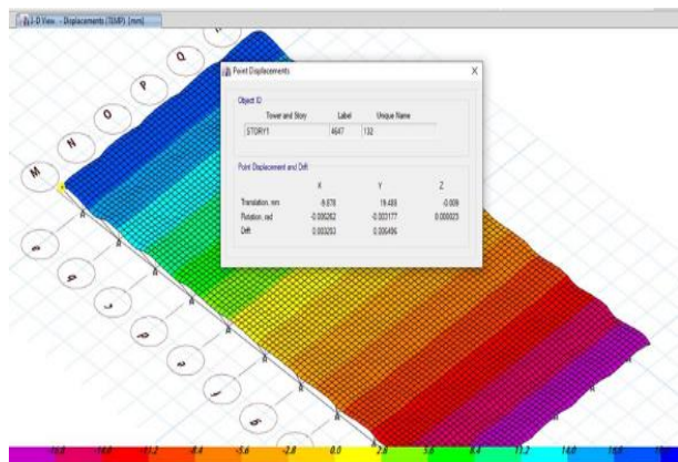
Fig. 7. Contours of slabs deformations under thermal loads.
