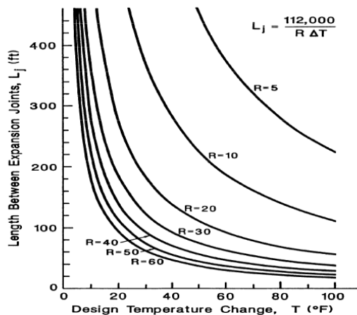
Fig. 1. Expansion joints separation for one-story concrete frame building versus variation in daily temperature [3].
