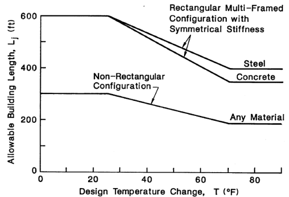
Fig. 2.The allowable spacing between building segments in feet [3].
