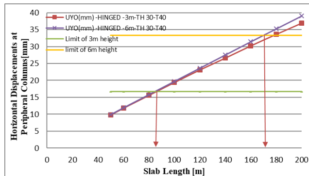
Fig. 9. Maximum spacing between joints for models with 30 cm slab thickness
