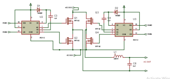
Figure 2 Hardware design of inverter
