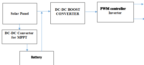
Figure 1 Block diagram
