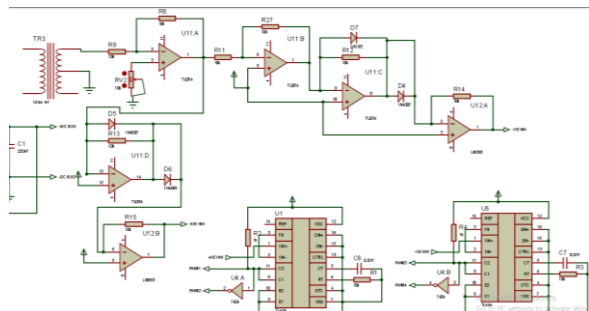
Figure 3 design for drive the the inverter circuit
