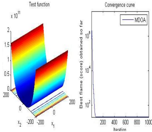
Figure 1. Unimodal Test Function and Convergence Curve of MDOA
