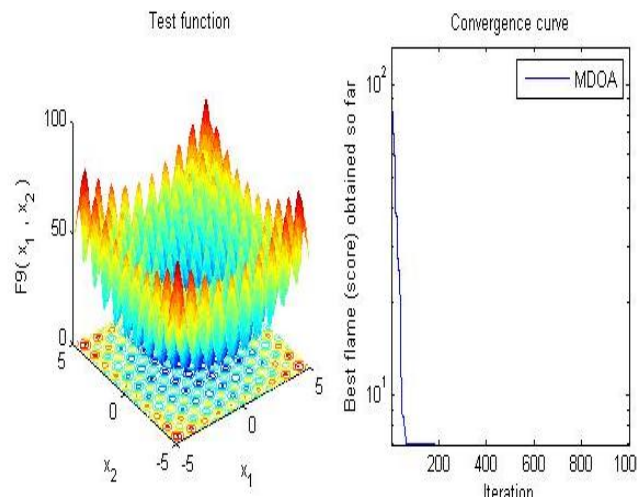
Figure 2. Multimodal Test Function and Convergence Curve of MDOA
