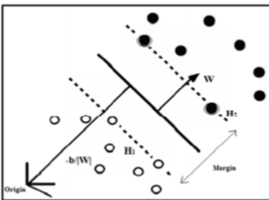
Fig.5.2 Maximum margin Hyper plane
