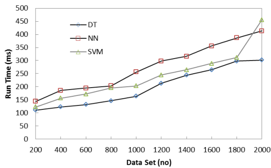
Fig.5.4 Runtime
