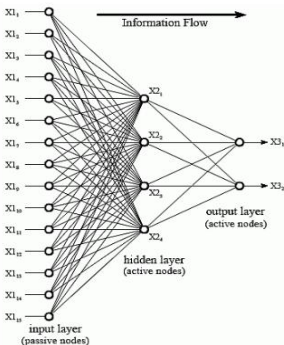
Fig.5.1 Neural Network
