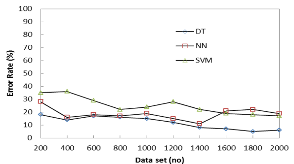
Fig.5.3 Error Rate
