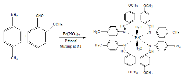
Scheme 4: In-situ synthesis of Schiff base [Pd(Anil-Tolu)_4(H_2O)_2] ligand
