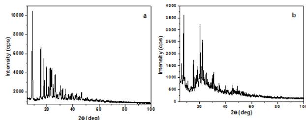
Fig.3. XRD spectra of Schiff base (a) and Schiff base Palladium metal complex
