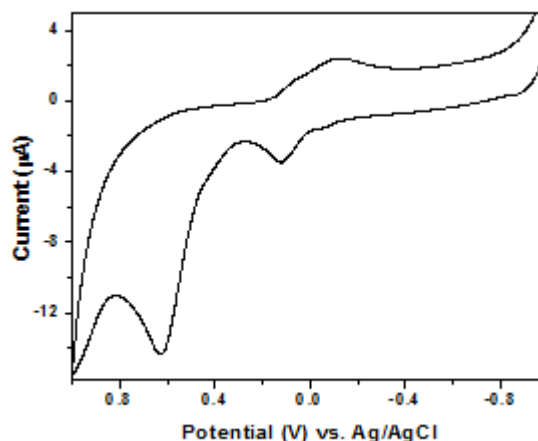
Figure 4. Cyclic voltammetry of Palladium Schiff base metal complex in 0.1 M PBS (pH 6) at scan rate 50 mV.
