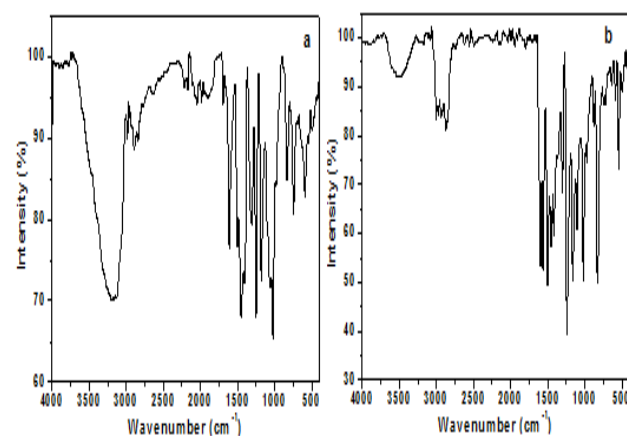
Fig.2. FT-IR spectra of Schiff base (a) and Schiff base Palladium complex
