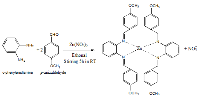
Scheme 2: In-situ synthesis of Schiff base [Zn(Anil-oPD) 4 ] ligand
