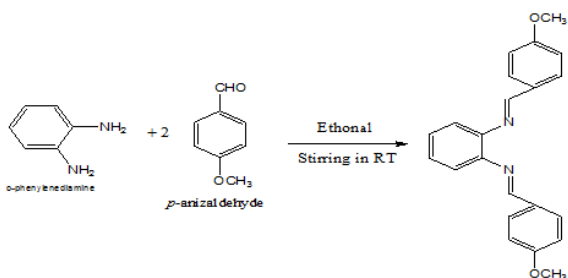
Scheme 1: In-situ synthesis of Schiff base [Anil-oPD] ligand
