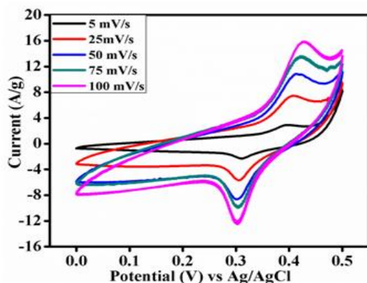
Fig. 3 CV curves of the CuO electrode material at different scan rate in 1M Na 2 SO 4 electrolyte
