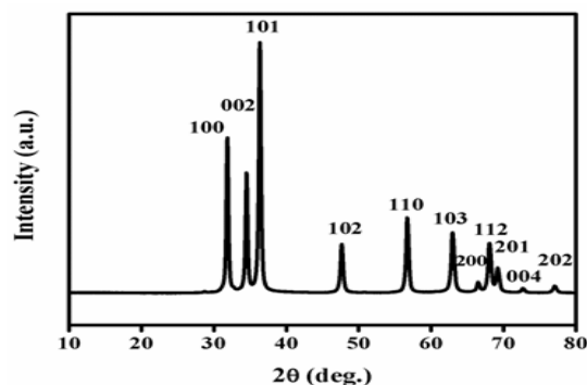
Fig. 1 XRD patterns of Pristine CuO nanorod
