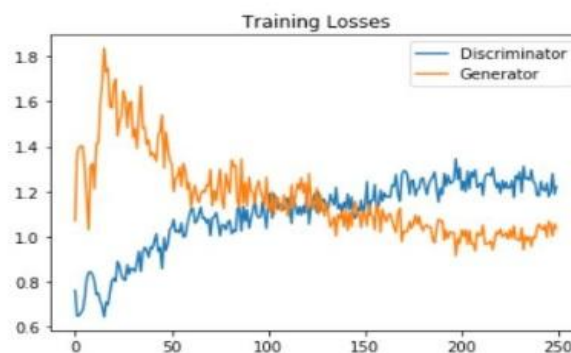
Fig 11 – The training Loss of Deep neural networks by Mohaksrivatsava et al
