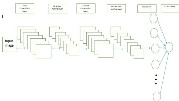
Fig 7. The Convolutional neural networks model
