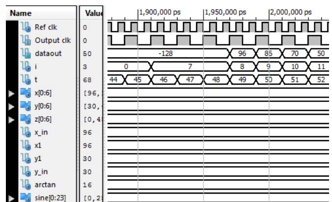
Fig. 2 Results of Discrete PLL Using LUT method
