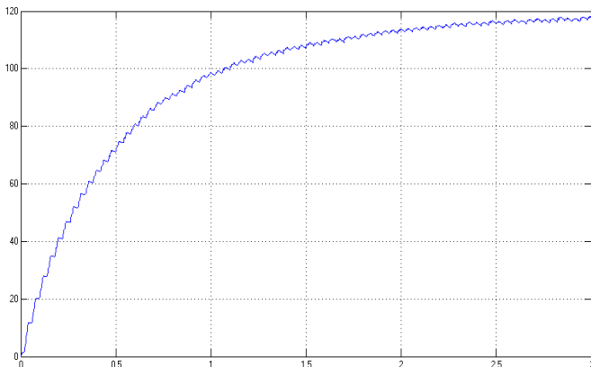
Figure 6. Output voltage of SEPIC Rectifier Voltage Doubler.
