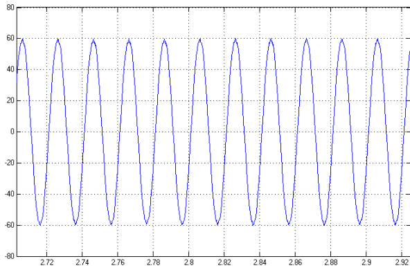
Figure 5. Input Voltage of SEPIC Rectifier
