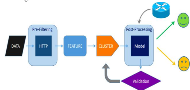
Figure. 3. Block Diagram of the proposed methodology.
