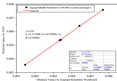
Fig. 9. PDF: Regression plot for obtained and predicted values
