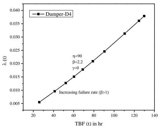
Fig. 7. The failure rate of dumper D4
