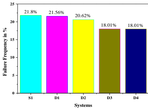
Fig. 6. Failure frequency of shovel and dumpers
