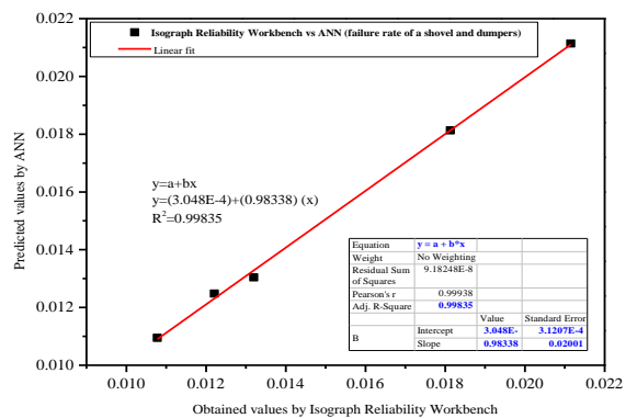
Fig. 10. Failure Rate: Regression plot for obtained and predicted values
