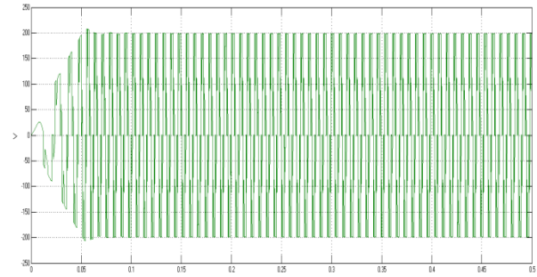
Fig5: BRUSH-LESS-DC motor input voltage response with their magnitude.
