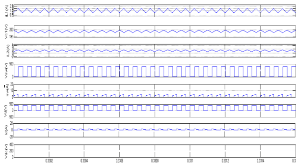
Fig8: \zeta dc-dc conversion device final working output with their response
