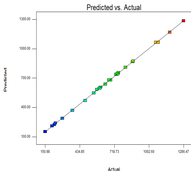
Fig. 5 Scatter plot of the observed values versus the predicted values
