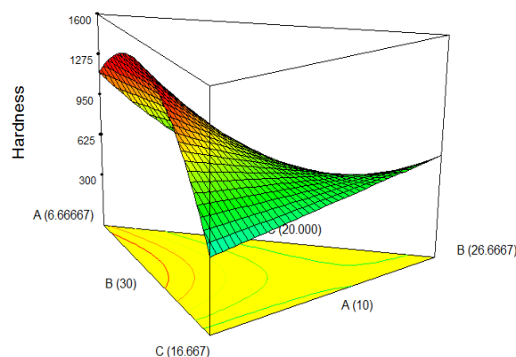
X 1 (A): Cocoa Butter; X 2 (B): Coconut oil; X 3 : Olive oil (C) Actual components: Palm oil (D): 9.167; water (E): 25.000; NaOH (F): 9.167
