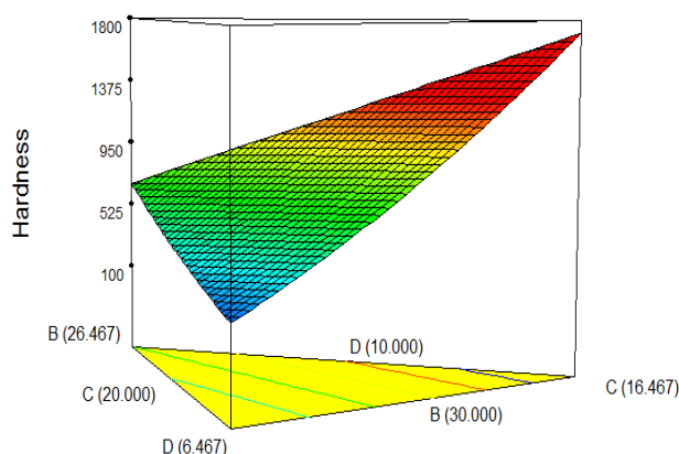
X 1 (B): VCO; X 2 (D): Palm oil; X 3 : Olive oil (C) Actual components: cocoa butter (A): 9.093; water (E): 24.723; NaOH (F): 9.717
