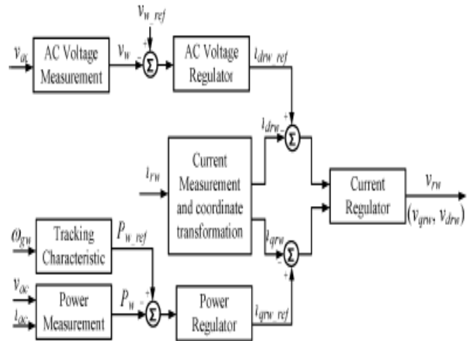
Fig. 6. Control block diagram for the RSC of the DFIG.
