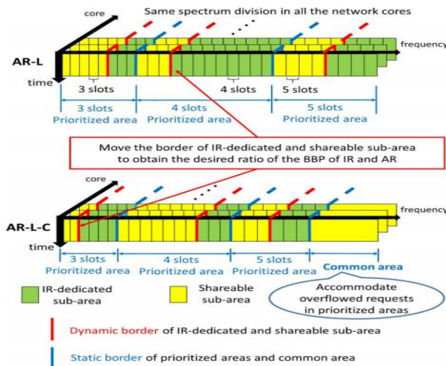
Fig. 3. Virtual resource design of the proposed methods. All the areas and sub-areas follow the same spectrum division in the network, including the core domain, due to the continuity constraint on the transmission route in RSA.
