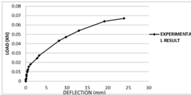
Fig: 3.3 graph of pile head deflection of long pile obtain from experimental result
