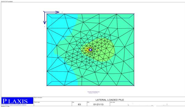
Fig.5.8 lateral loaded pile obtained by Plaxis -3D - Foundation
