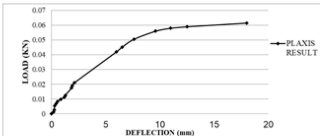
Fig:5.3 Pile head deflection of SHORT pile obtained from Plaxis value
