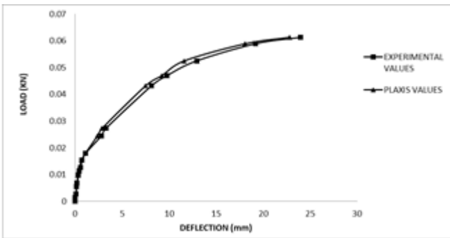
Fig. 6.1 Graph represent the comparison between experimental value and plaxis values for short pile
