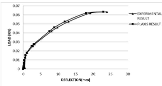
Fig. 6.2 Graph represent the comparison between experimental values and plaxis values for INTERMEDIATE pile
