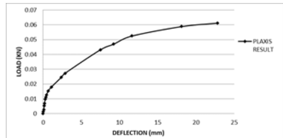
Fig: 5.5 Pile head deflection of LONG pile by using Plaxis result
