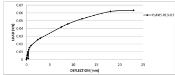
Fig: 5.4 Pile head deflection of INTERMEDIATE pile by using Plaxis result
