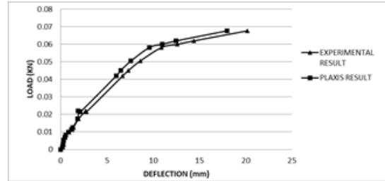
Fig. 6.3 Graph represents the comparison value for experimental result and plaxis result for LONG pile.
