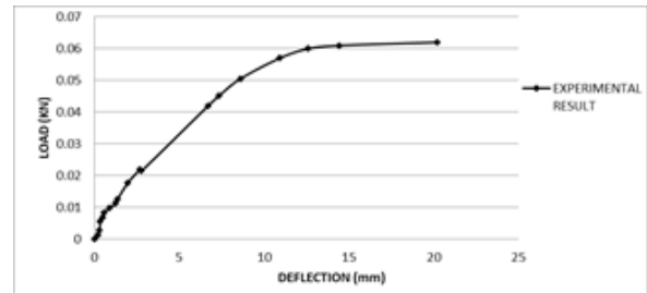
Fig: 3.1 Pile head deflection of short pile obtain from experimental result
