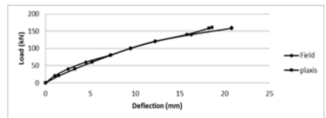
Fig: 4.1 Comparison between the finite element result and field test data
