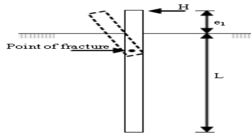
Fig: 5.6 sketch diagram of deflected pile head
