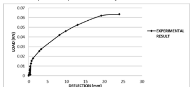
Fig: 3.2 Pile head deflection of intermediate pile obtained from experimental result
