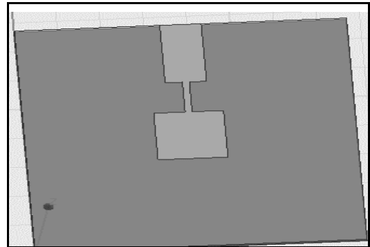
Fig 8: Square type-2 Antenna with stub feedline
