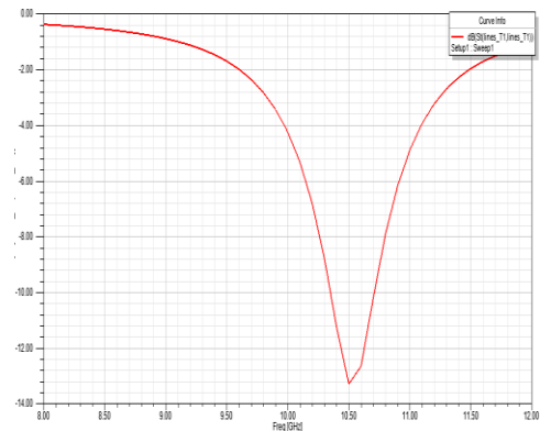
Fig 3: Bandwidth and Reflection coefficient of Rectangular type-1 Antenna
