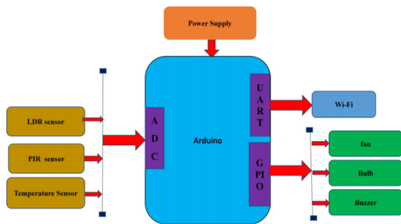
Fig.4. Block Diagram
