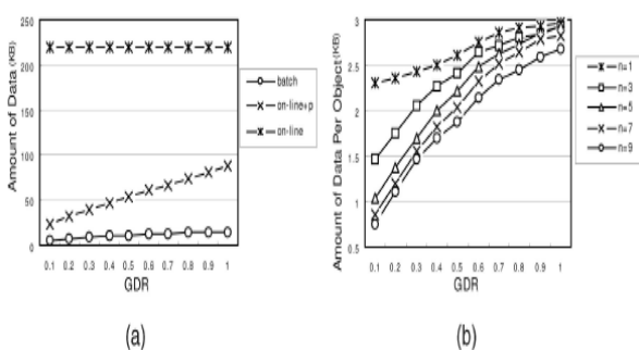
Figure 6. Performance comparison of with respect to different objects present in WSNs
