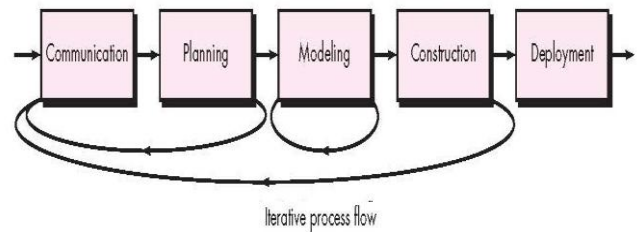
Fig. 3 Iterative model [7]
