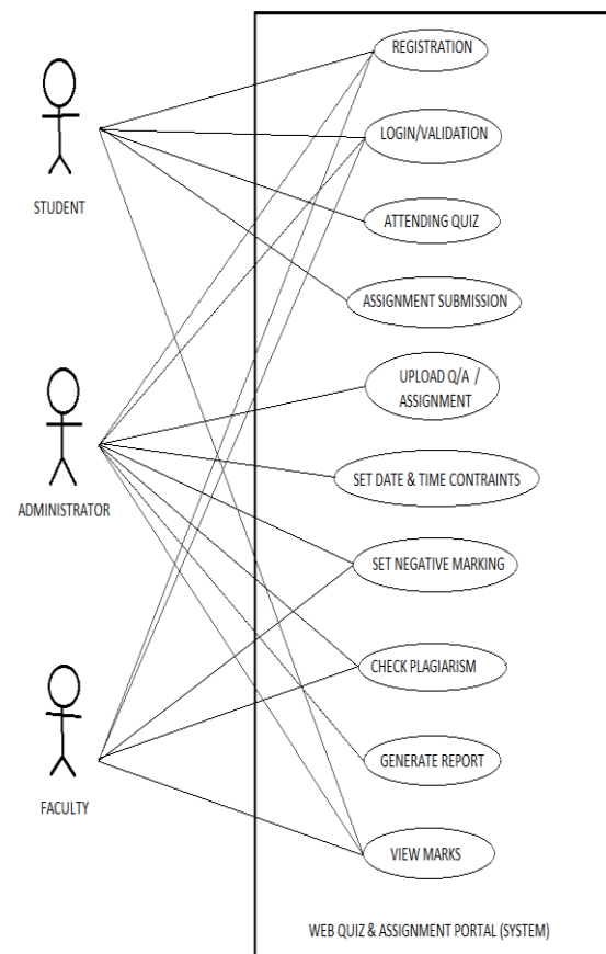
Fig. 1 Use Case Diagram
