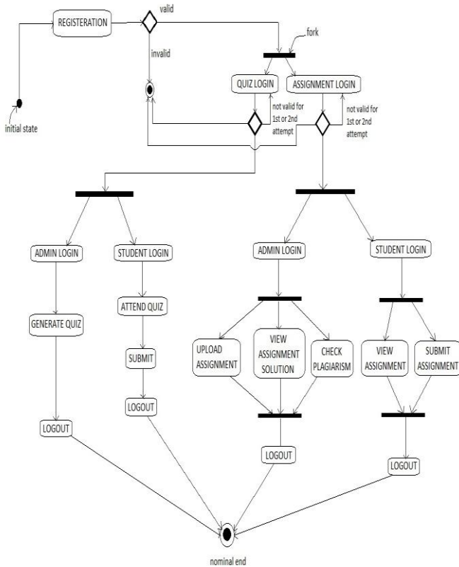
Fig. 2 Activity Diagram
