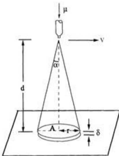
Fig. 2. Flow rate determination
