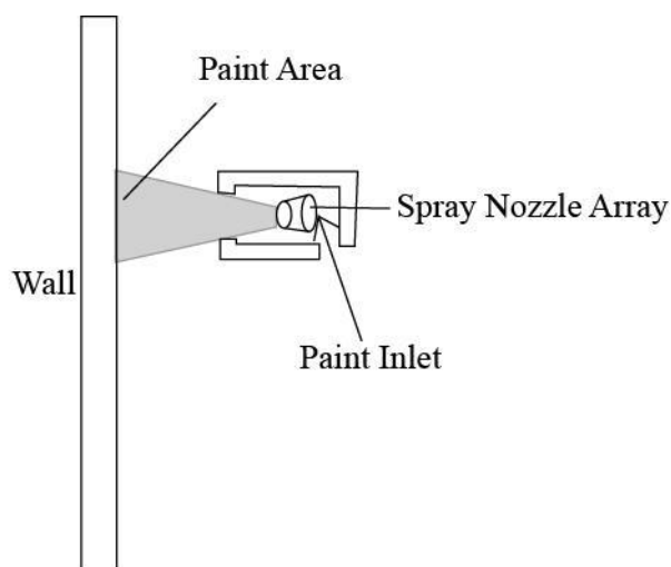
Fig. 5. Paint Spray Nozzle
