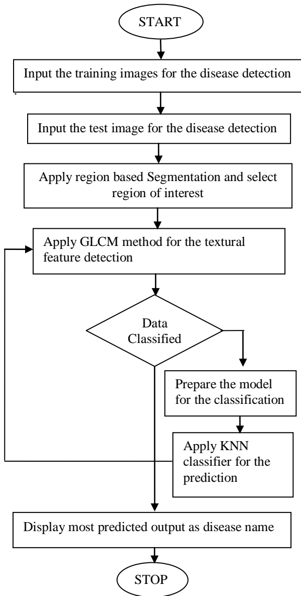
Fig. 1: Proposed Flowchart
